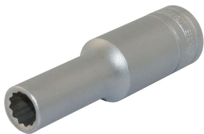
1/2" Drive Deep 12 Point Socket 22mm
